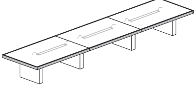
CX1663 L539 P120 H75 CX1680 L707 P120 H75
